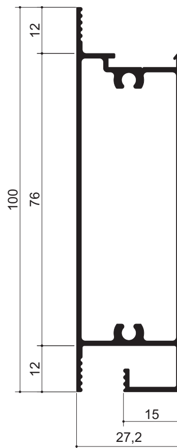
PME-078 Marco/Travessa 1,045 Kg/m
