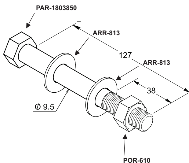
PAR-1803850 Parafuso 3/8" x 5" ARR-813 Arruela 3/8" POR-610 Porca 3/8"
