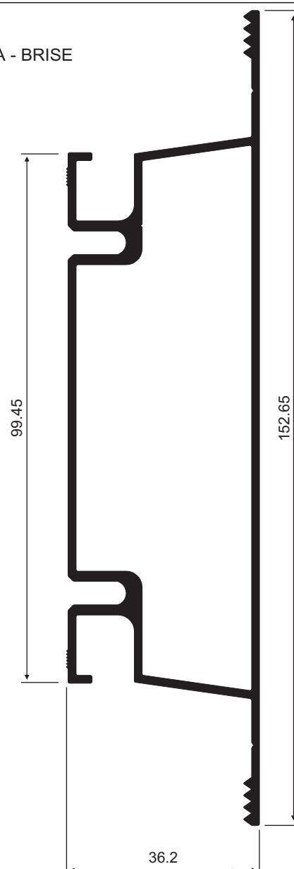
PFS-222 1,782 Kg/m
