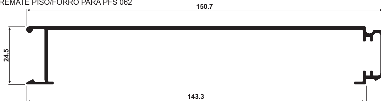
PFS-162 0,983 Kg/m
