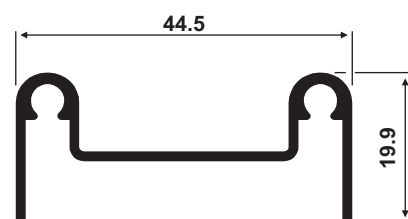
PFS-174 0,408 Kg/m
